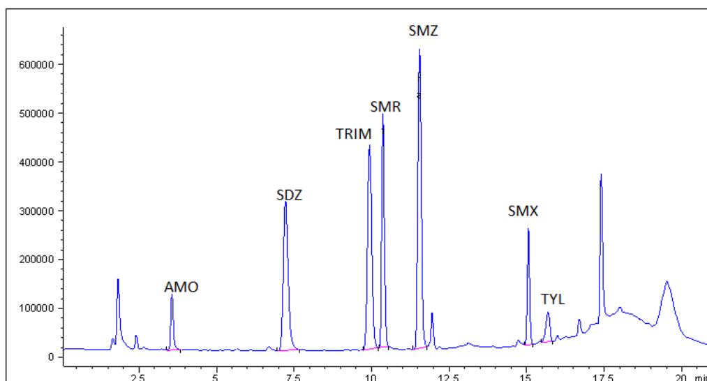
Fig. 2. Selected-ion monitoring chromatogram of feed matrix spiked with all analysed antibacterial substances at first validation level
