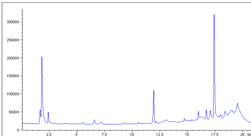
Fig. 1. Selected-ion monitoring chromatogram of blank feed sample
